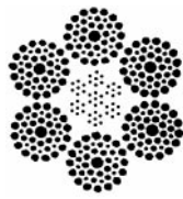
6 x 41 Warrington Seale (7 x 7 IWRC)
