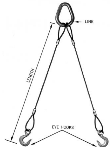
Press-Grip Sling/Type U-6
