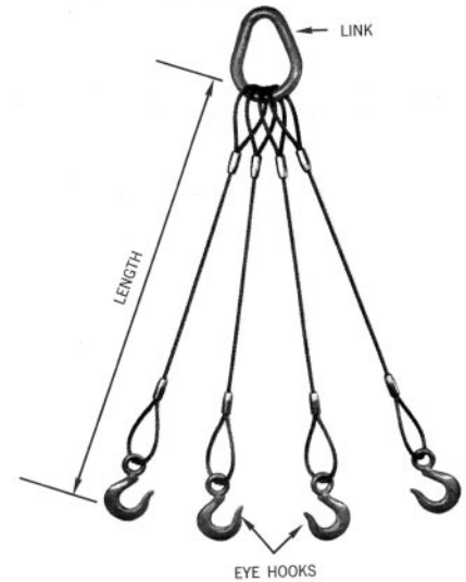
Press-Grip Sling/Type U-8
