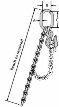
Style A
