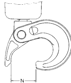
Latchlok Type Hook
