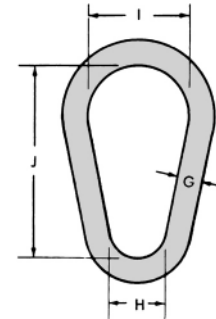
CM Pear-Shaped Master Link
