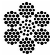
6 x 19 Warrington (1 x 19 Strand Core)
