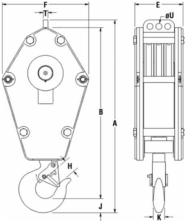
McKissick® 380 Series Easy Reeve® Crane Block Dimensions
