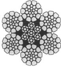
Flex-X 6
