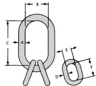
CM Oblong Master Link Sub-Assembly
