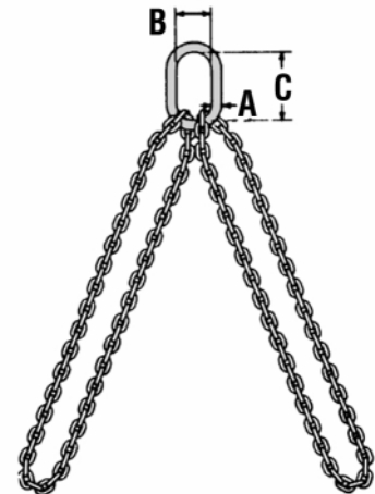
Double Endless Basket
