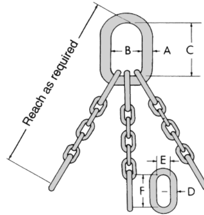
CM Standard Triple Branch Magnet Chains
