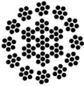
19 x 7
