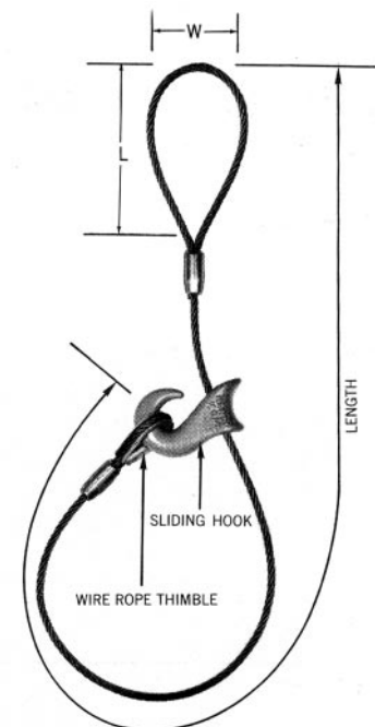
Press-Grip Sling / Type U-3
