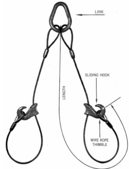
Press-Grip Sling/Type U-4
