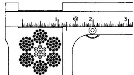
Incorrect
