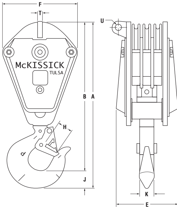
McKissick Utility Crane Block — 383 — Triple
