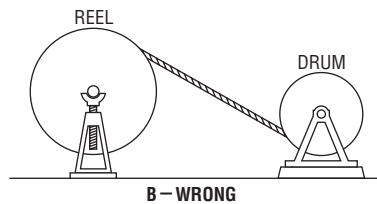
The correct (A) and the wrong (B) way to wind wire rope from reel to drum.
