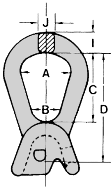
CM Bail-Type Magnet Chain Assemblies
