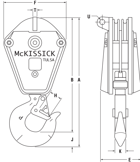
McKissick Utility Crane Block — 382 — Double
