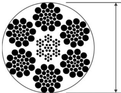
True Diameter
