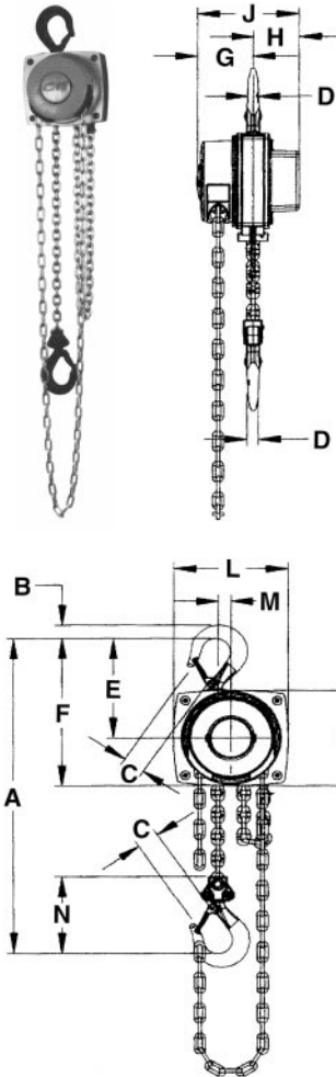
CM Hurricane Hand Chain Hoist
