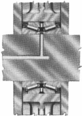
Double Row Sealed Tapered Roller Bearing
