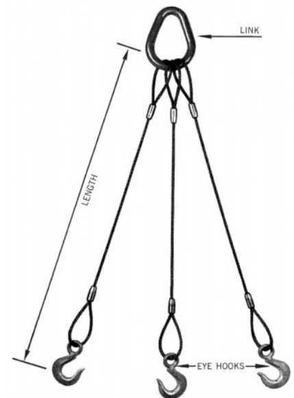
Press-Grip Sling/Type U-9
