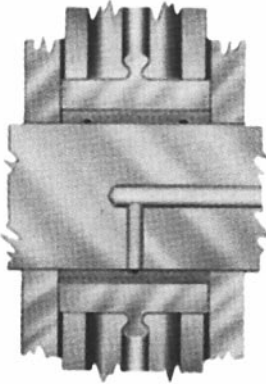
Bronze Bushed — S.A.E. 660 Bronze with Figure "8" Oil Groove
