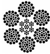
6 x 36 Warrington Seale (7 x 7 IWRC)
