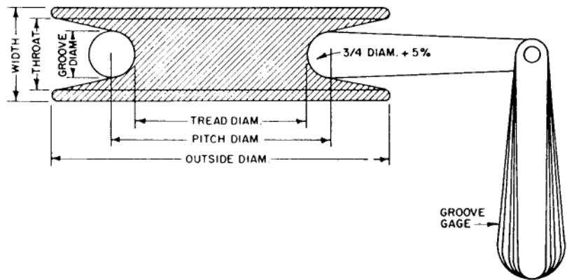
Illustrating the various dimensions of a sheave, and the use of a groove gage.
