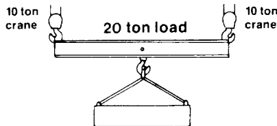
Team Two Cranes of Equal Capacity
