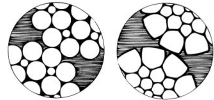
6 x 26 WS and Flex-X
