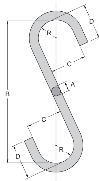
CM S Hook
