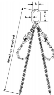
Style B
