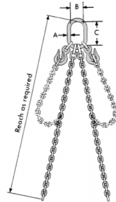
Style A
