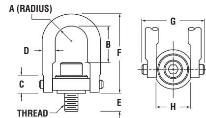
Actek Safety Hoist Ring
