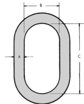
CM Oblong Master Link
