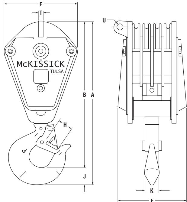
McKissick Utility Crane Block — 384 — Quad
