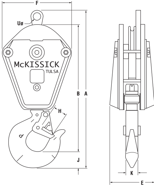
McKissick® Utility Crane Block — 381 — Single
