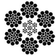
6 x 26 Warrington Seale (7 x 7 IWRC)
