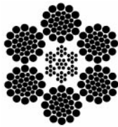
6 x 31 Warrington Seale (7 x 7 IWRC)
