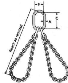
Double Basket Type
