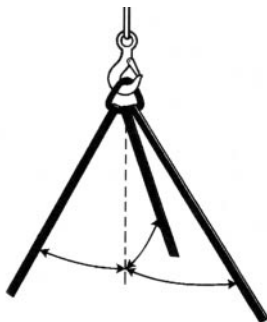
Sling Angle of 45°
