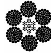
6 x 49 SWS (Seale Warrington Seale)
