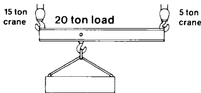
Custom Beam Design Allows Teaming Two Cranes of Unequal Capacity
